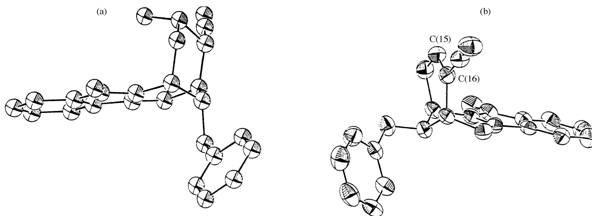
Fig. 2 (a) X-Ray crystal structure of the TMS-protected alcohol 21b , ‡ with the TMS group removed for clarity. (b) X-Ray crystal structure of the \alpha,\beta -unsaturated nitrile 22 , § where the position of the double bond was confirmed by the C(15)–C(16) bond length of 1.332(8) Å.
