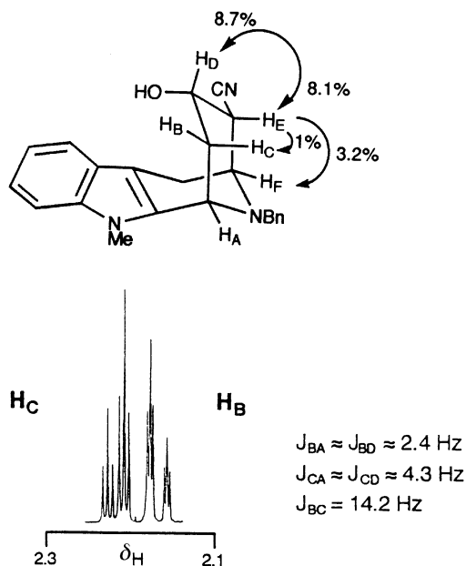
Fig. 1 Selected NMR data for 21a (NOEs and ^1\text{H} NMR) indicating the relative stereochemistry
