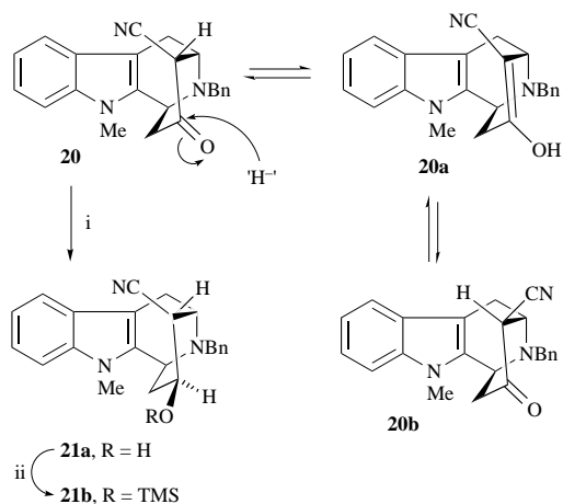
Scheme 7 Reagents and conditions: i, \text{NaBH}_4 , MeOH, room temp., 2 h; ii, \text{Me}_3\text{SiCl} , \text{CH}_2\text{Cl}_2 , imidazole, -10^\circ\text{C} to room temp., 1 h
