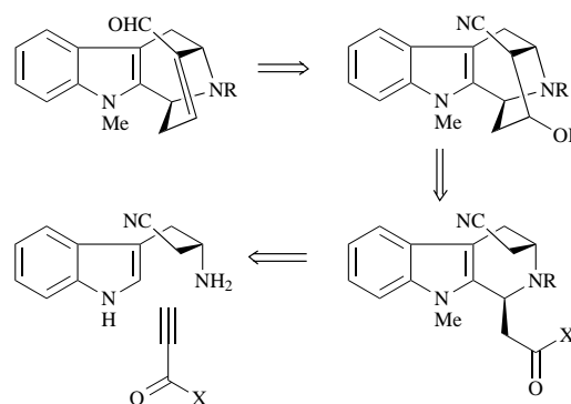
Scheme 2 Retrosynthetic analysis of route to bridged indole alkaloids
