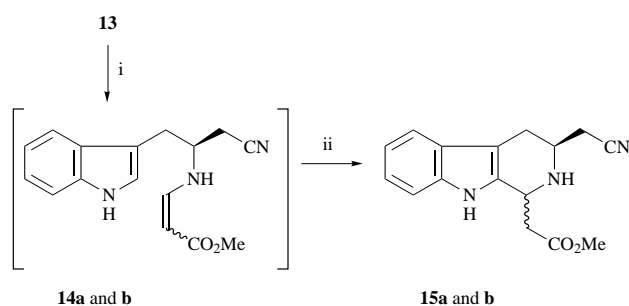
Scheme 4 Reagents and conditions: i, methyl propynoate, CHCl 3 , reflux, 100 h; ii, cool to 0 °C, and add TFA (2 equiv.), 30 min
