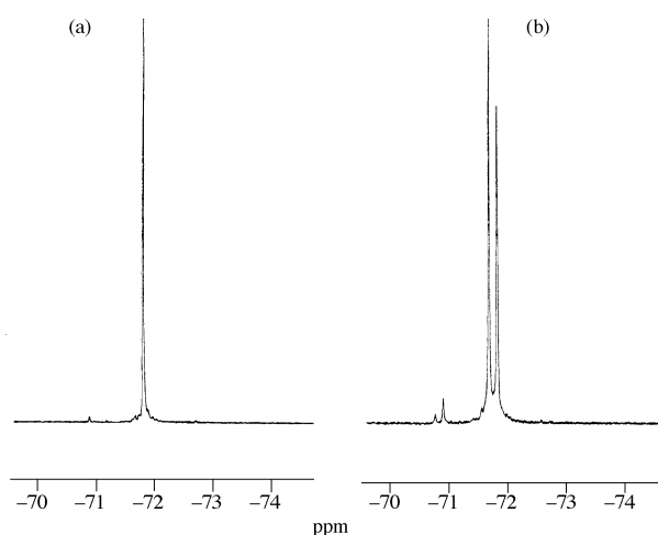
Fig. 3 (a) ^{19}\text{F} NMR of ( R )-Mosher's ester 23a (crude product). (b) ^{19}\text{F} NMR of ( R )- plus ( S )-Mosher's esters 23a and 23b , for assignment of peaks. Spiking experiments allowed quantification of the diastereoisomeric peaks and confirmed the ee of (–)- 10 to be >97%.
