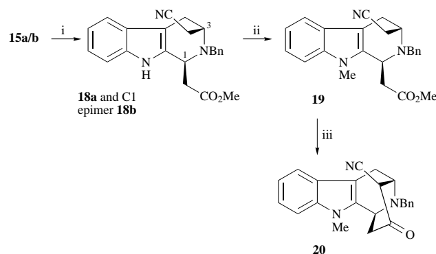
Scheme 6 Reagents and conditions: i, BnBr, NaHCO 3 , CH 2 Cl 2 , reflux, 96 h; ii, MeI, NaH, DMF, room temp., 30 min; iii, LiNEt 2 , THF, –78 °C, 1 h
