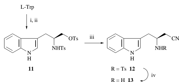
Scheme 3 Reagents and conditions: i, LAH, THF; ii, TsCl, pyridine; iii, KCN, MeOH; iv, Na, NH 3 (liq.)
