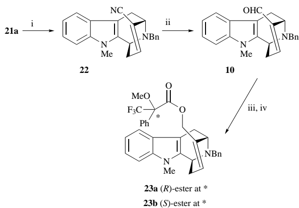
Scheme 8 Reagents and conditions: i, \text{POCl}_3 , pyridine, benzene, reflux, 48 h; ii, DIBAL, \text{CH}_2\text{Cl}_2 , -78^\circ\text{C} (30 min) to room temp. (5 h); iii, \text{NaBH}_4 , MeOH, room temp., 2 h; iv, ( R )- or ( S )- \text{PhC}(\text{OMe})(\text{CF}_3)\text{COCl} , pyridine, \text{CH}_2\text{Cl}_2 , room temp.
